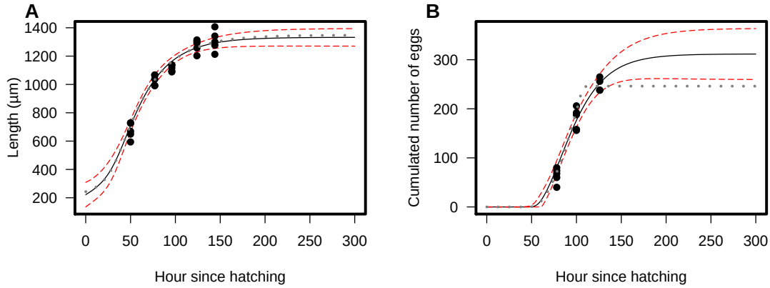
Figure IX.1: C. elegans length ( A ) and cumulated reproduction ( B ) in relation to age (hour since hatching) for the control conditions. Observed data are represented by points , the model fits (Eq. IX.1) are represented by the regression line . Dashed lines represent the 95% confident interval of the model ( CI = Mean \pm 1.96 \times \sigma ). Dotted lines represent the model fitted with the equations of Jager et al. (2005).
